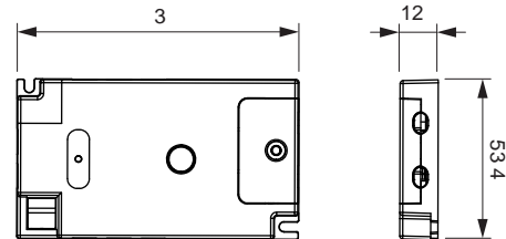
Control Box
