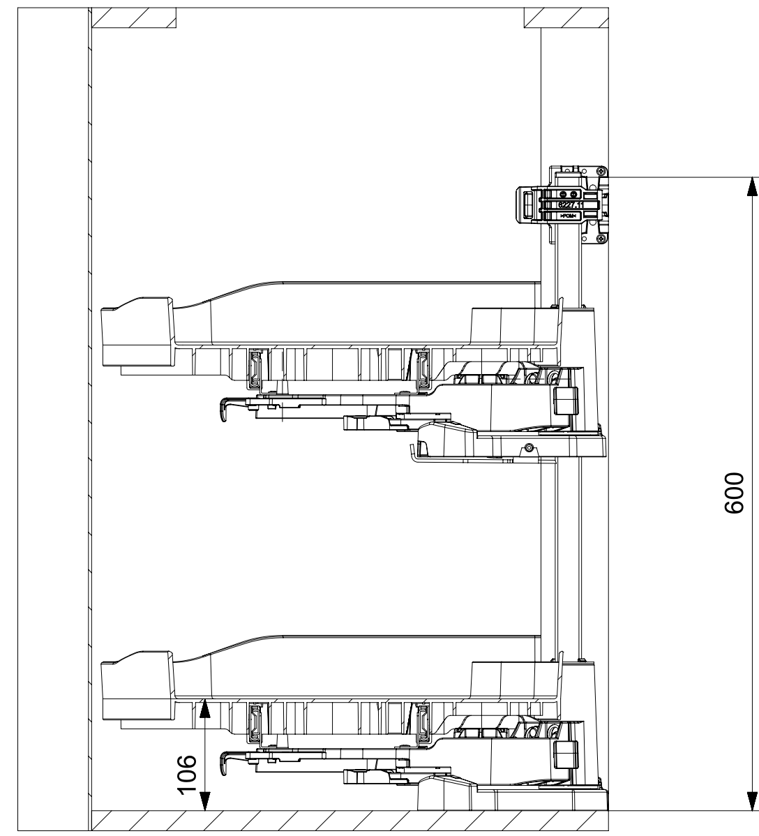
SECTION E-E
