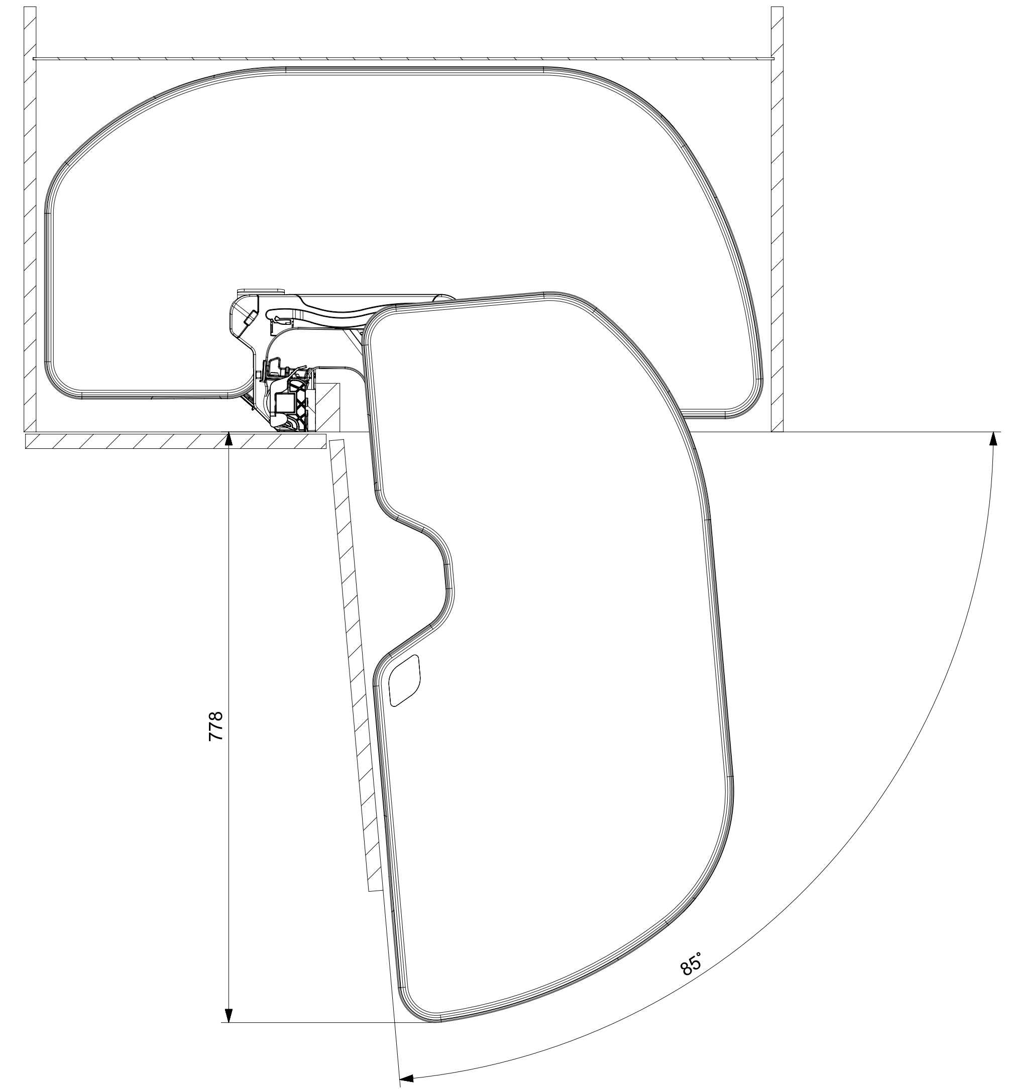
SECTION G-G
